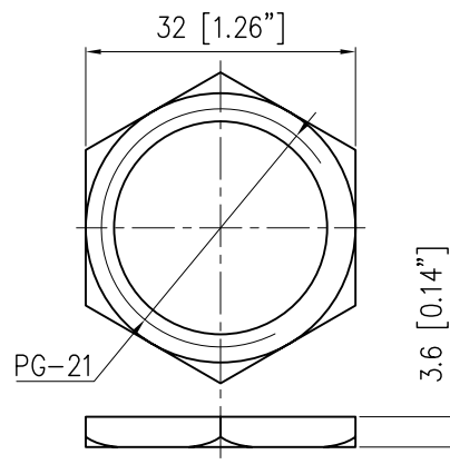
NUT PG-21
