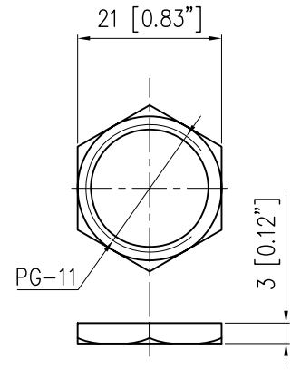
NUT PG-11
