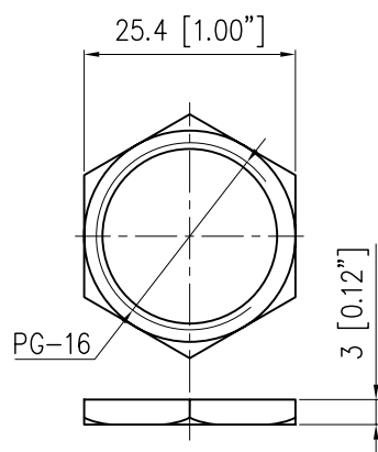
NUT PG-16
